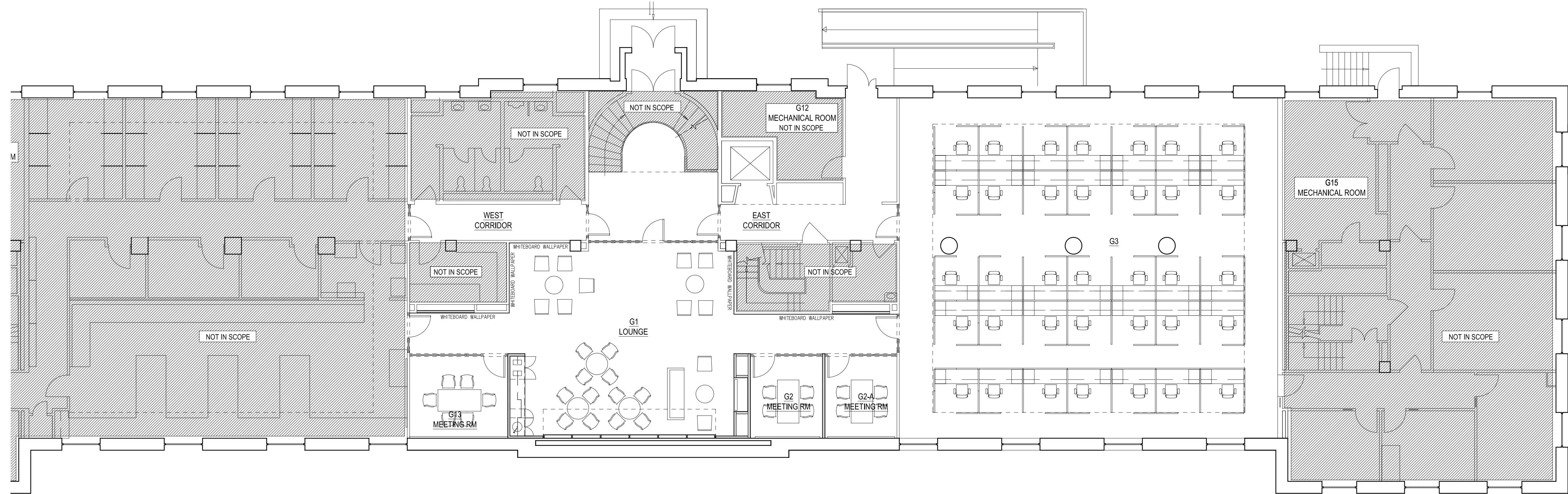
1 PROPOSED FURNITURE PLAN 1/8" = 1'-0"
